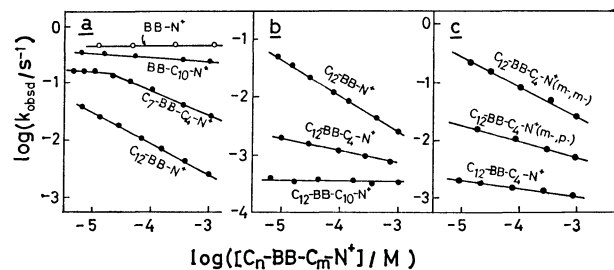
Fig. 4. Concentration dependence of the rate constant. 30 °C, pH 5.5 \pm 0.1 (0.02 M phosphate buffer), \mu = 0.02 (KCl).
